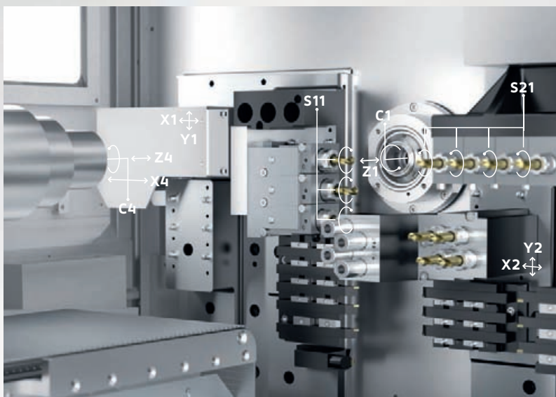
Swiss ST 26
